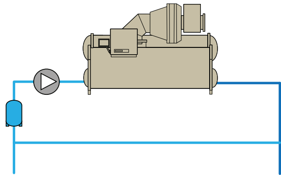
Figure 16. Chilled fluid loop buffer tank upstream of chiller and downstream of decoupler
