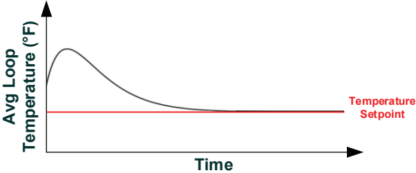
Figure 4. Continuous unloading compressor in a system with higher loop volume
